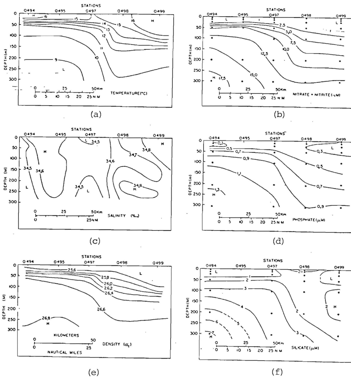
Fig. 33. Vertical distribution of physical and chemical properties for the transverse plume section: a) temperature ( ^{\circ}\text{C} ), b) nitrate-nitrite ( \mu\text{M} ), c) salinity ( ^{\circ}/\text{oo} ), d) phosphate ( \mu\text{M} ), e) density ( \sigma_t ), f) silicate ( \mu\text{M} ).
