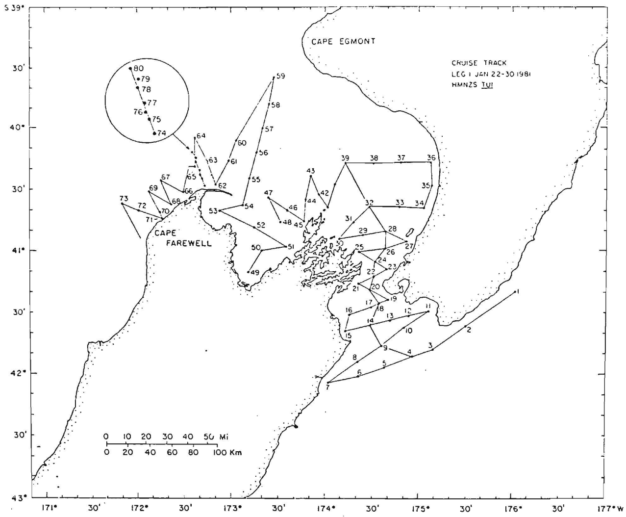
Fig. 16. Cruise track and station positions for leg 1, January 22- 30, 1981.
