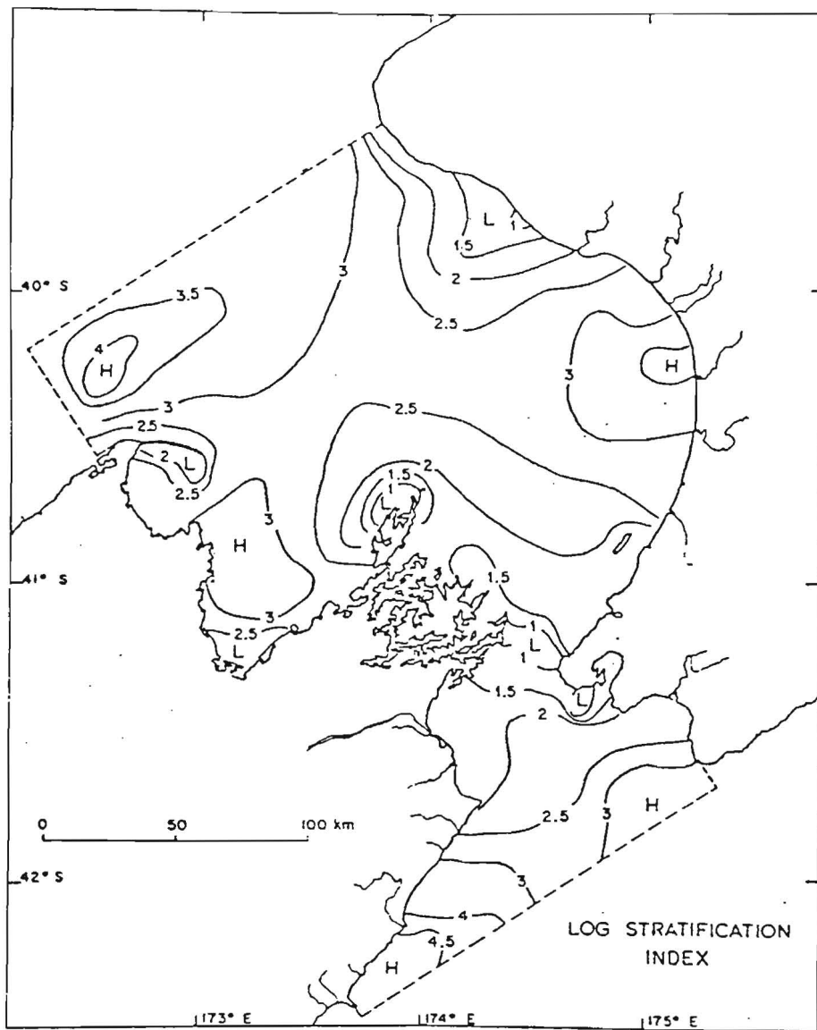
Fig. 3. Contours of the log stratification index ( \text{m}^2 \text{sec}^{-3} ) derived from numerical model of Bowman et al. (1980).
