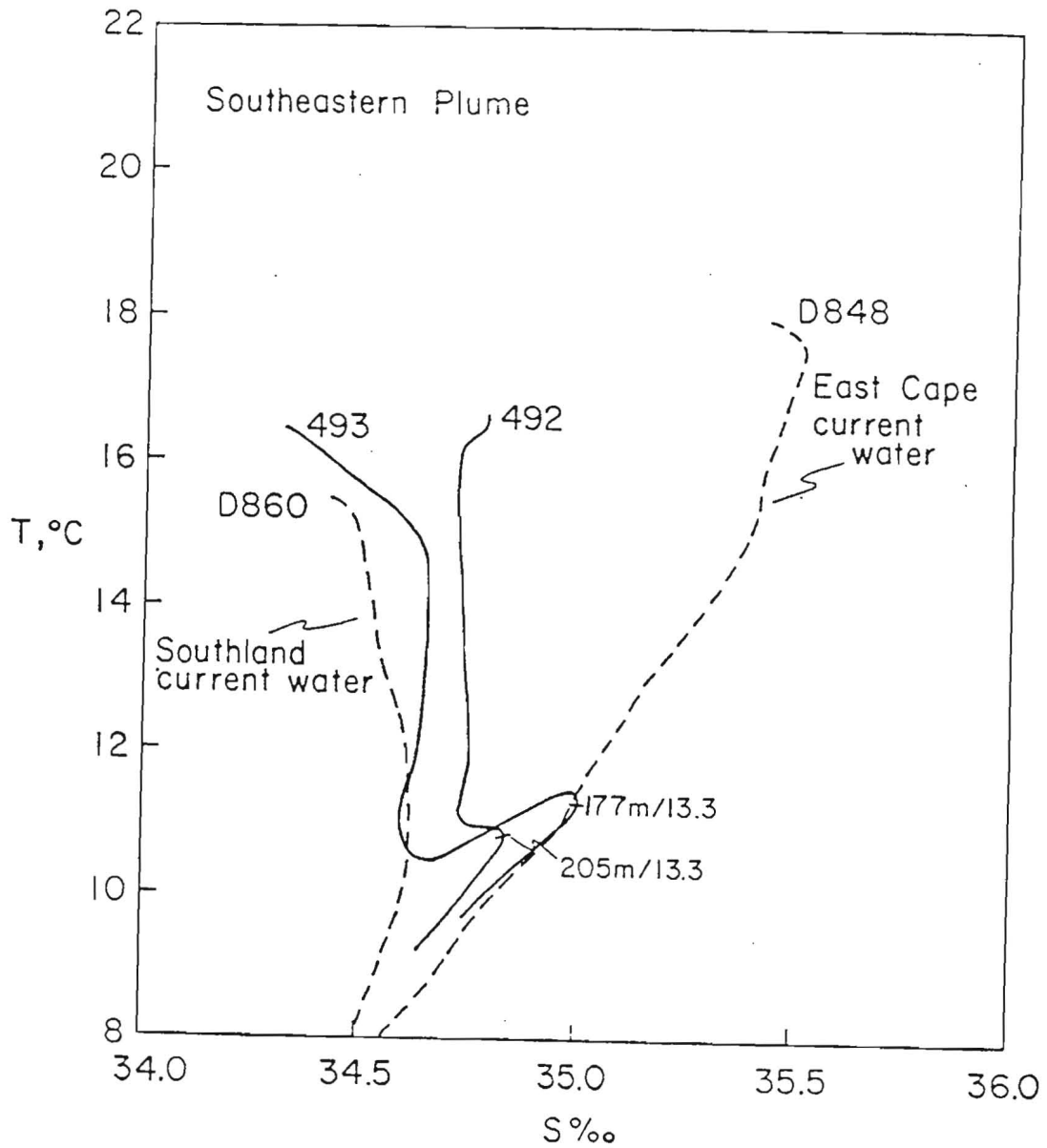
Fig. 36. Temperature-salinity diagram for the southeastern section of the plume, (Bowman et al. , in press c).
