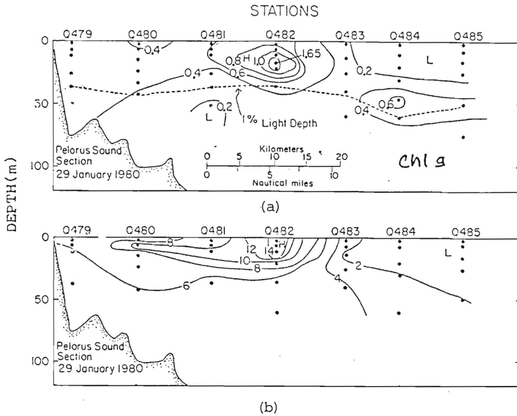
Fig. 15. Vertical distribution of biological properties for Pelorus Sound transect: a) chlorophyll 'a' ( \text{mg m}^{-3} ), b) primary production ( \text{mg C m}^{-3}\text{hr}^{-1} ), (courtesy P. Lapennas).
