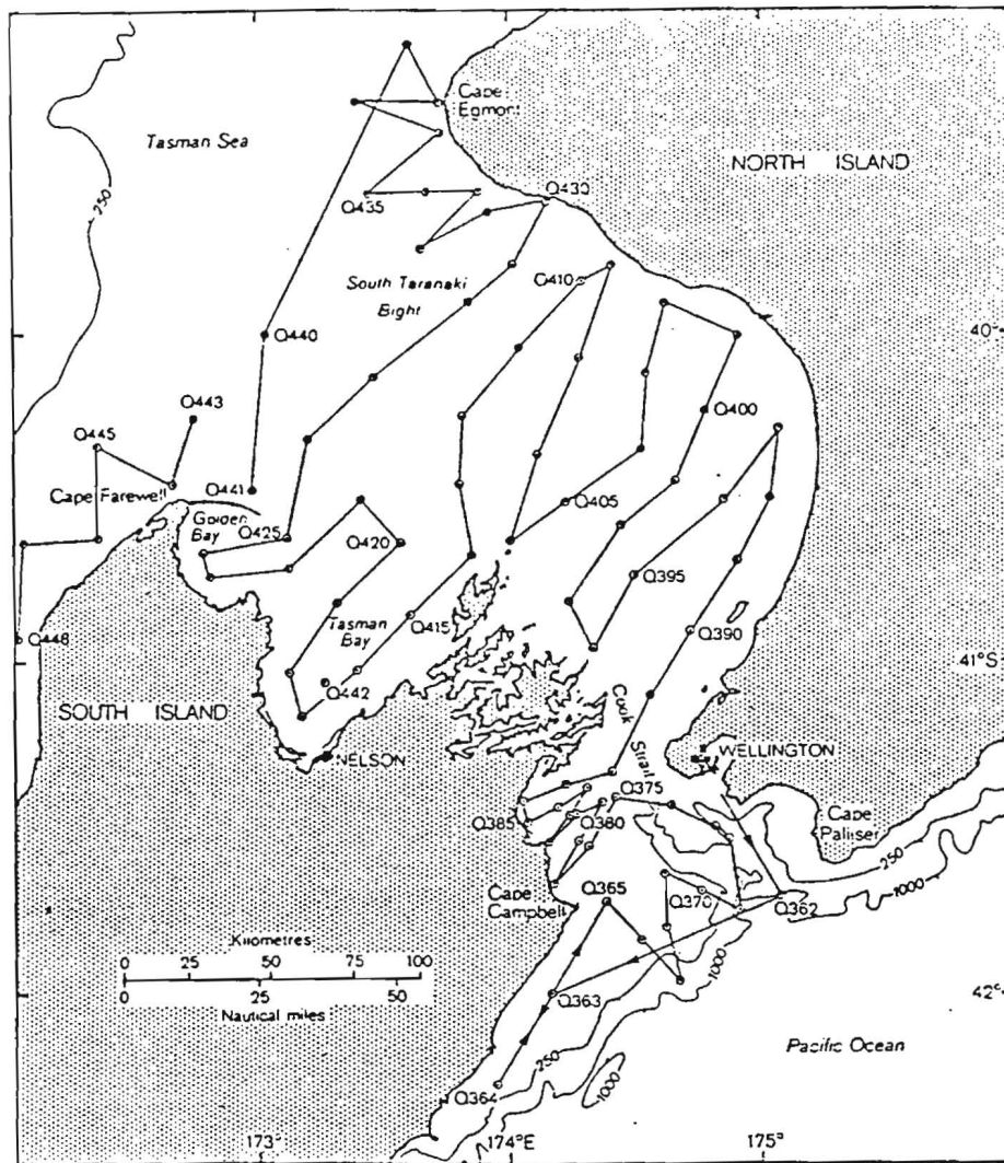
Fig. 4. Cruise track and station positions for leg 1, January 9-19, 1980
