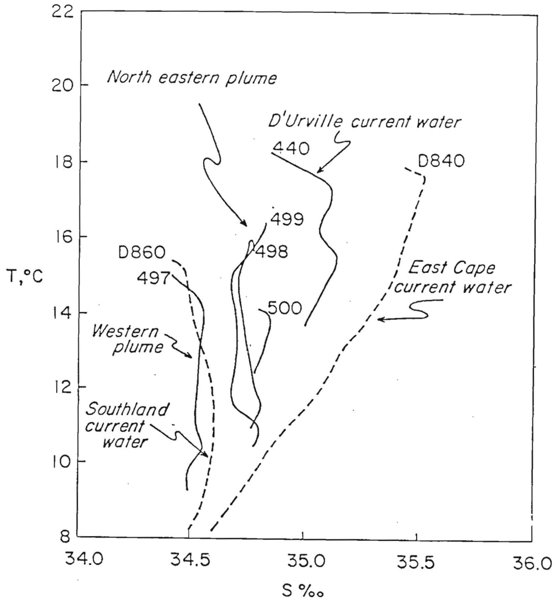
Fig. 23. Temperature-salinity diagram for the north-eastern section of the plume, January-February, 1980, (Bowman et al. , in press c).
