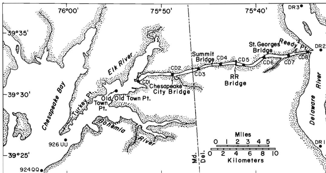
Fig. 6. Chart of Chesapeake and Delaware Canal showing location of temperature, salinity and suspended sediment stations.
