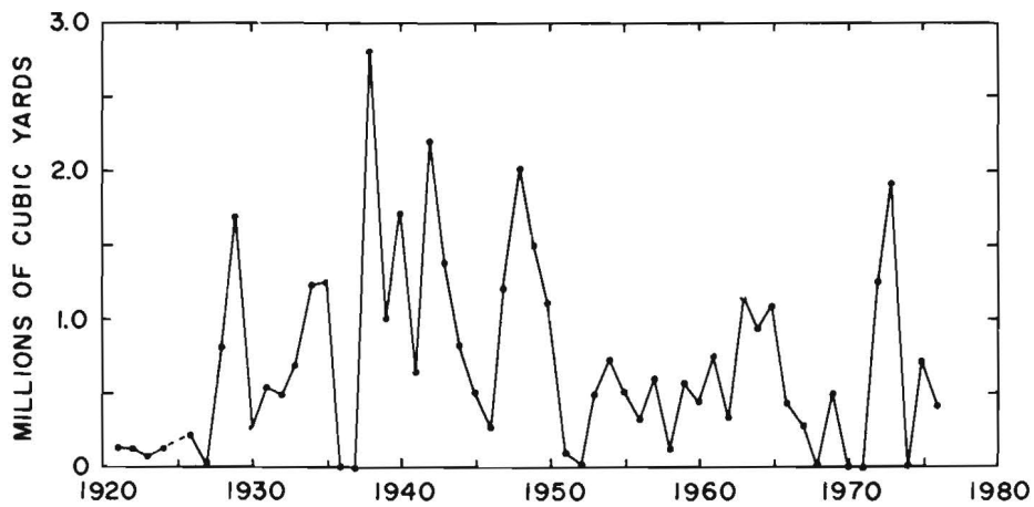
Fig. 4. Volume of maintenance dredging in Chesapeake and Delaware Canal, 1921-1976.
