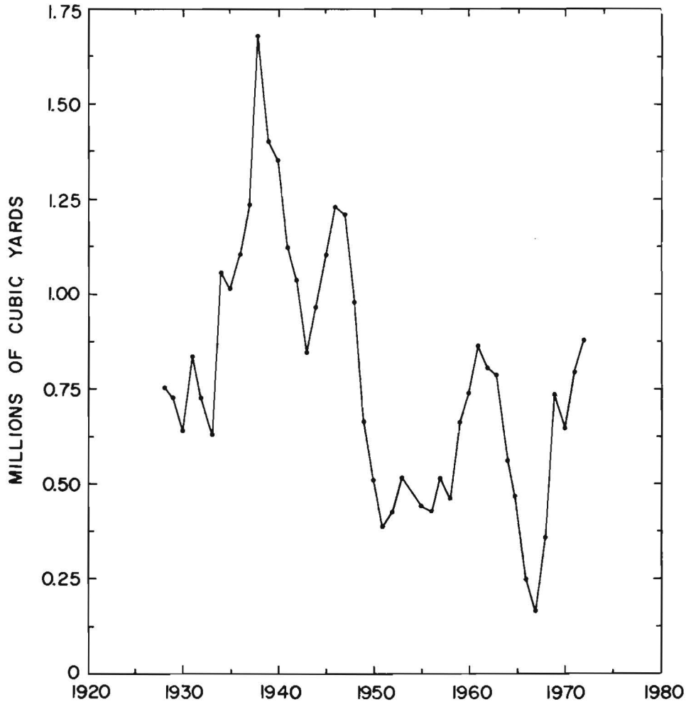
Fig. 5. Volume of maintenance dredging in Chesapeake and Delaware Canal, 1928-1972, by five-year rolling average.
