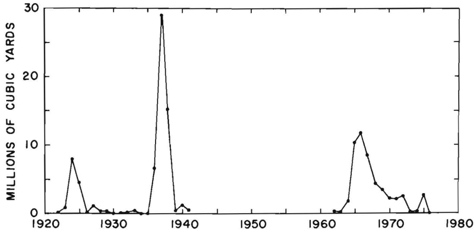
Fig. 3. Volume of improvement dredging in Chesapeake and Delaware Canal, 1921-1976.
