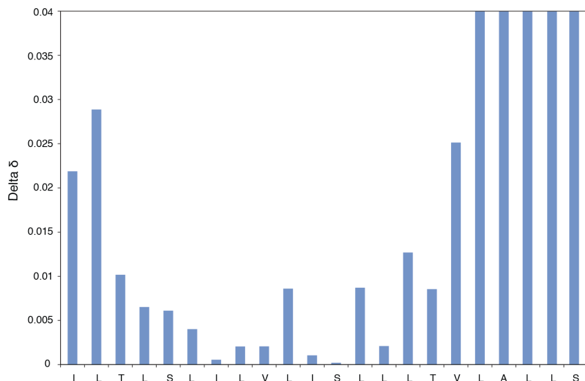
Figure 4.4 Chemical shift differences of the TM domain between muEpoR 220-248 and muEpoR 218-268 . The core residues of the TM domain, including the dimer interface residues S231, V235, S238, and T242 remain in the same position, an indication of conformation preservation.
