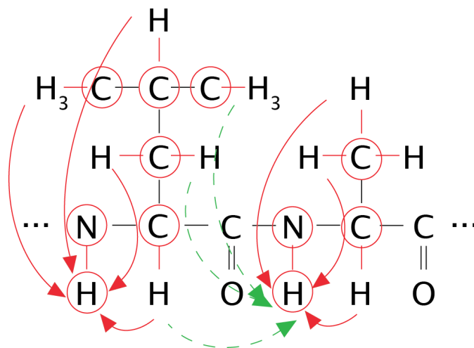
Figure 2.11 The ^{13}\text{C} - ^{15}\text{N} -NOESY experiment (aka. HSQC-NOESY-HSQC). This experiment measures through-space contacts between the amide proton and protons attached to carbons, but records the chemical shift of the carbon atom instead of the proton.
