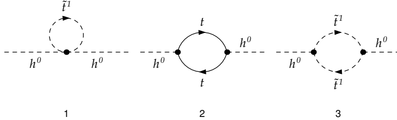
Figure C.2: Top/stop contribution to Higgs self energy
