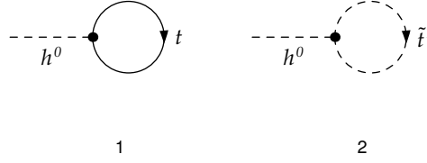
Figure C.1: Top/stop contribution to Higgs tadpole diagrams
