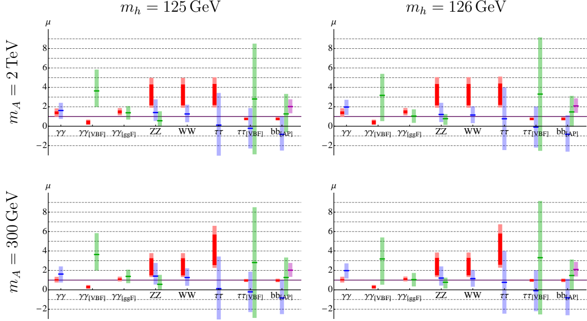
Figure 5.2: Comparing the signal strength predictions for each Higgs decay channel of electroweak baryogenesis in the MSSM with the ATLAS, CMS and Tevatron data as explained in Section 5.4.1. Subscripts indicate exclusive production via a single mode. For each channel we show up to three bands: the EWBG prediction, with m_{\tilde{\tau}_R} \in (80, 115) GeV (red, with theoretical error bands in light red) and the ATLAS/CMS 1\text{-}\sigma best-fit measurements (blue/green, with central value indicated in dark blue/green). In the bb_{[AP]} channel we also show the combined Tevatron constraint as a fourth band (purple). The SM prediction is indicated with a horizontal line at \mu = 1 .
