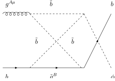
Figure D.7: Box diagram, B_3 .
