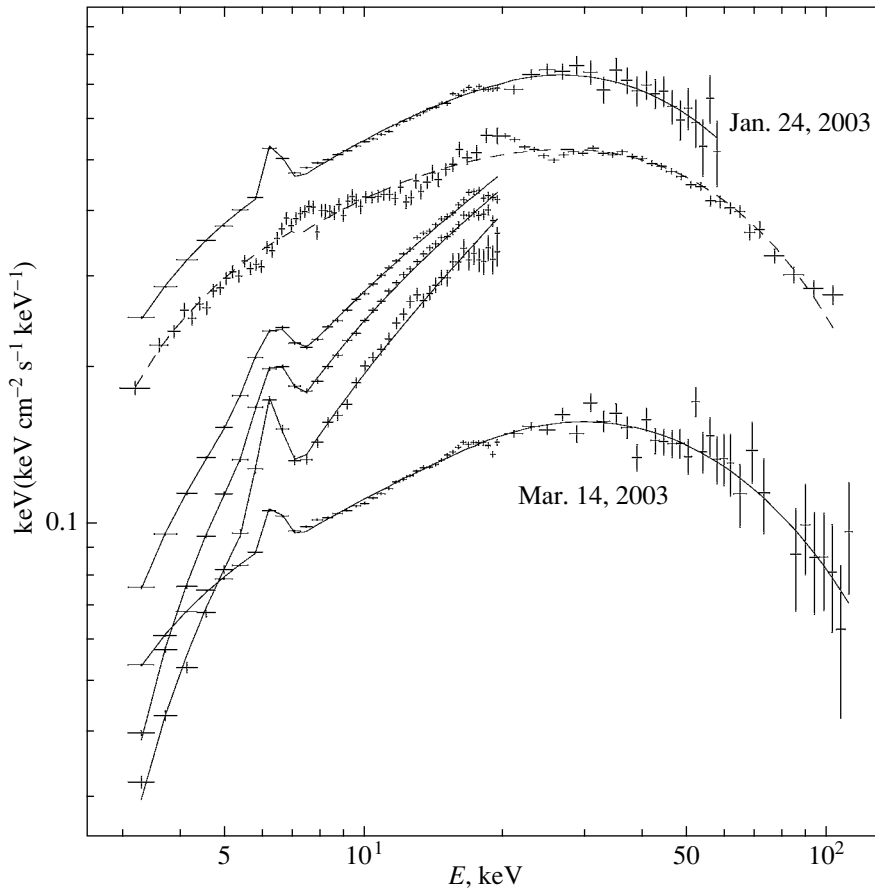
Fig. 4. Persistent spectra for MX 0836–42 constructed from the data of the JEM-X and ISGR/IBIS telescopes aboard the INTEGRAL observatory (dashed line) and the PCA (3–20 keV) and HEXTE (20–60 keV) detectors aboard the RXTE observatory (solid lines). For convenience of perception, the values of these spectra and the model in the spectrum for March 14, 2003, were multiplied by a factor of 1/3.
